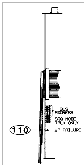
Figure 8-2 IEEE 488 Module Top View
