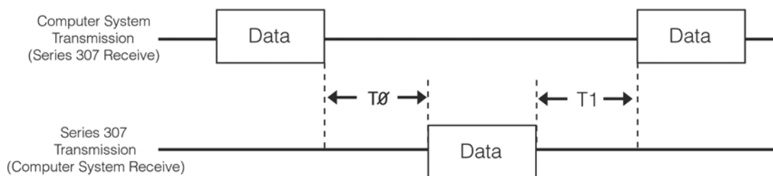
Figure 7-5 RS-485 Data Timing
