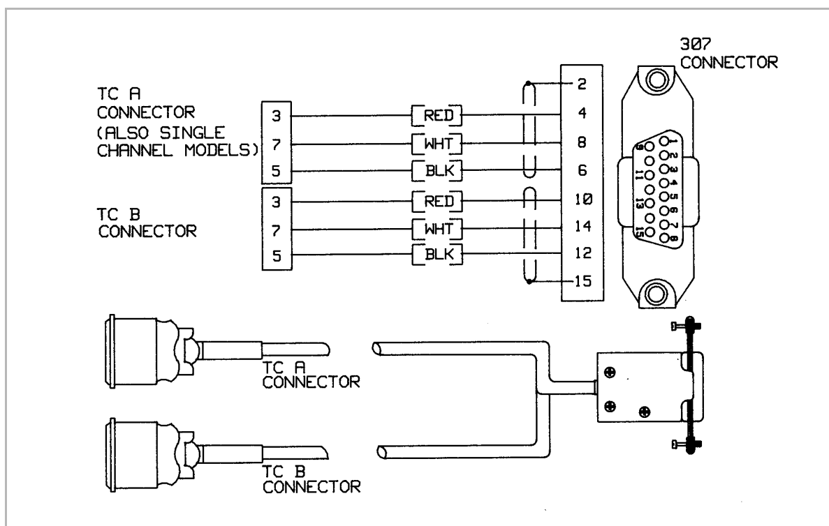
Figure 11-6 Thermocouple Gauge Cable
