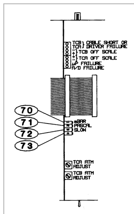
Figure 4-1 Thermocouple Module, Top View.
