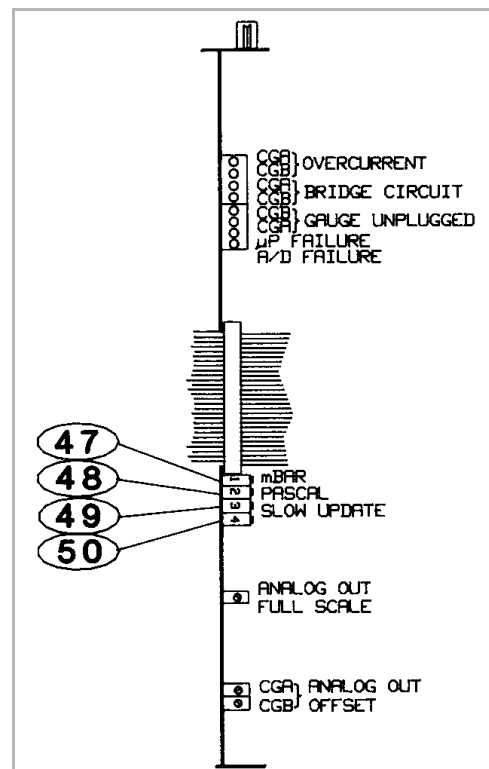
Figure 3-1 Convectron Module, Top View.
