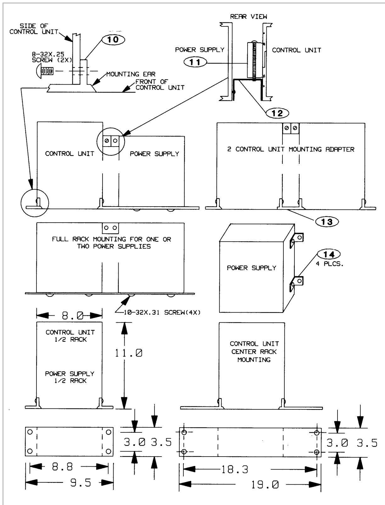
Figure 1-5 Mounting Methods.
