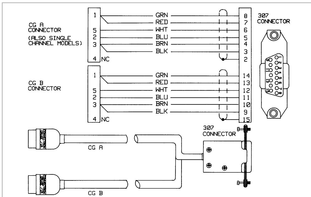
Figure 11-5 Convectron Gauge Cable
