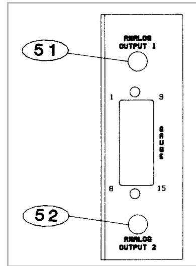
Figure 3-9 Convector Module Rear panel.
