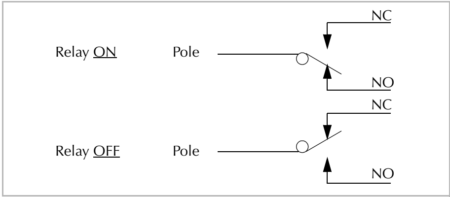
Figure 5-5 Process Control Relay Contacts Status.
