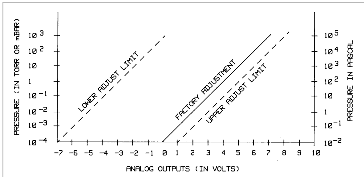
Figure 3-10 Convector Gauge Pressure Analog Output.
